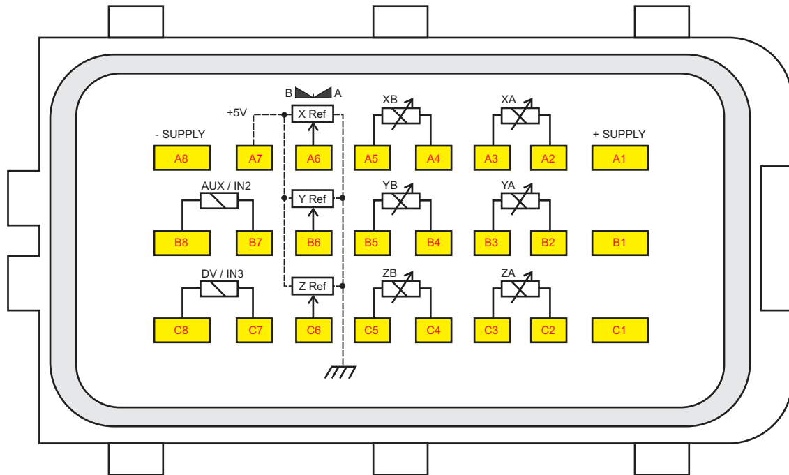
Male 24 way connector
